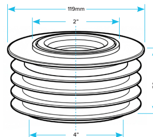
2" Drain Connector Reducer
