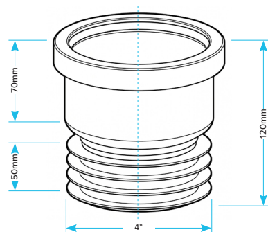
4" Straight 1/2" Boss Drain Connector
