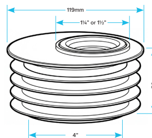
1/4" or 1/2" Offset Drain Connector Reducer
