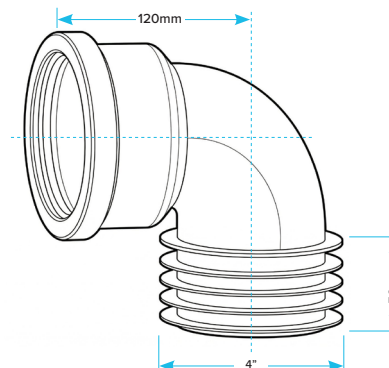
4" 90 Angle Drain Connector
