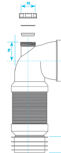
90° Flexible Pan Connector (32mm Adapter)
