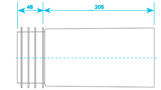
Extension WC Pan Connector
