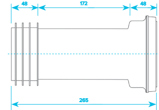
Extended Straight WC Pan Connector
