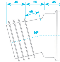
14° Angle WC Pan Connector
