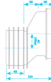
40mm Offset WC Pan Connector
