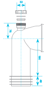
90° Bend WC Pan Connector (32mm Adapter)
