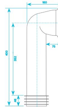
90° Bend Long Tail WC Pan Connector
