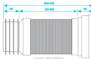
Long Flexible Pan Connector
