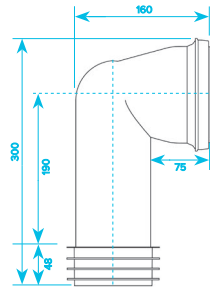
90° Bend WC Pan Connector
