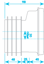
20mm Offset WC Pan Connector
