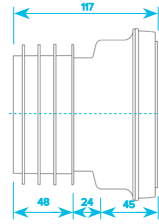
Straight WC Pan Connector
