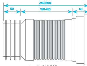
Medium Flexible Pan Connector
