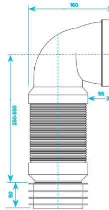
90° Flexible Pan Connector
