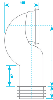
Swan Neck WC Pan Connector
